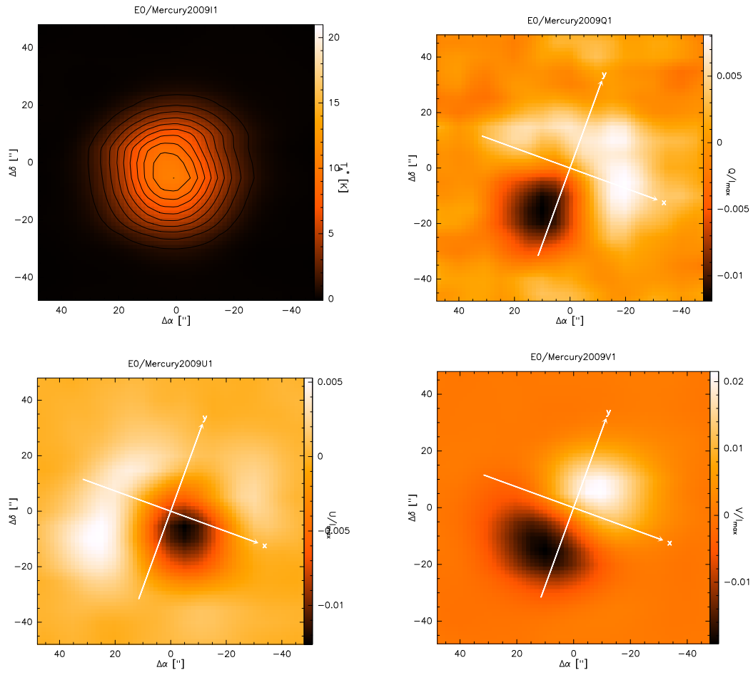
Figure 1: Stokes maps obtained on 03-Sep-2009 with EMIR (band E0LI) from Mercury (size = 8.7") at 86 GHz. The rotation angle is \chi_0 = 25.0^\circ .
