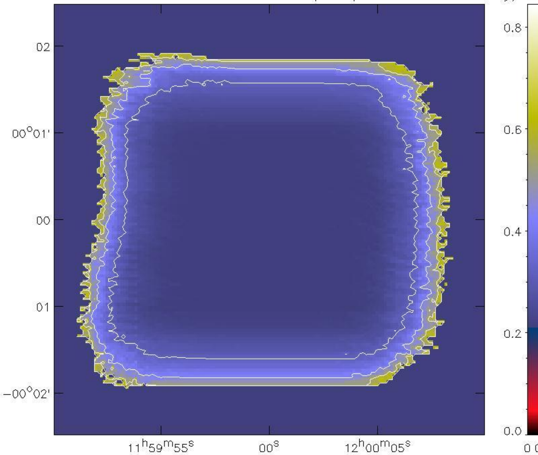
Noise 1mm RF Azel Map: Neptune
