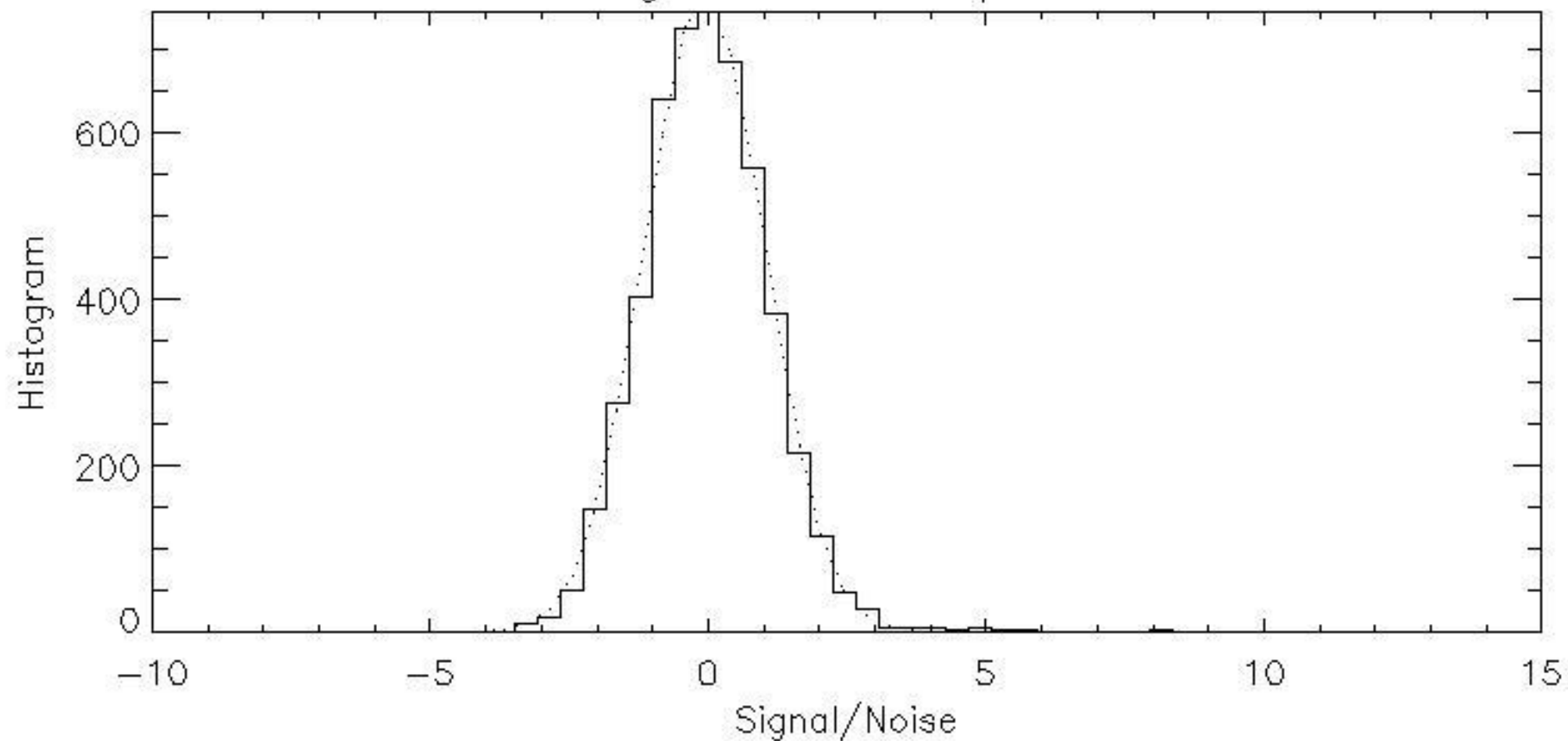
Average RFA Azel Map: GMAur
