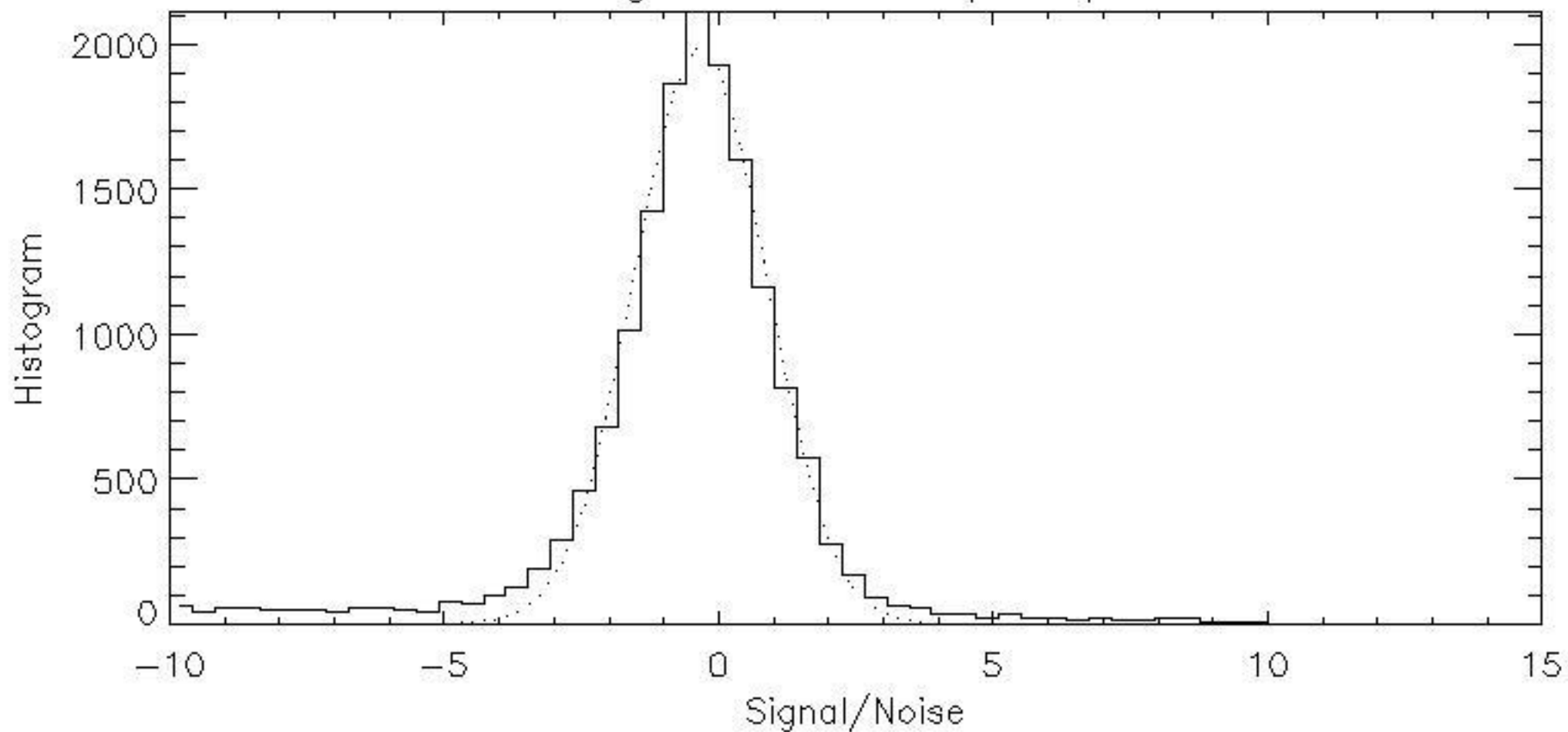
Average RFB Azel Map: Neptune
