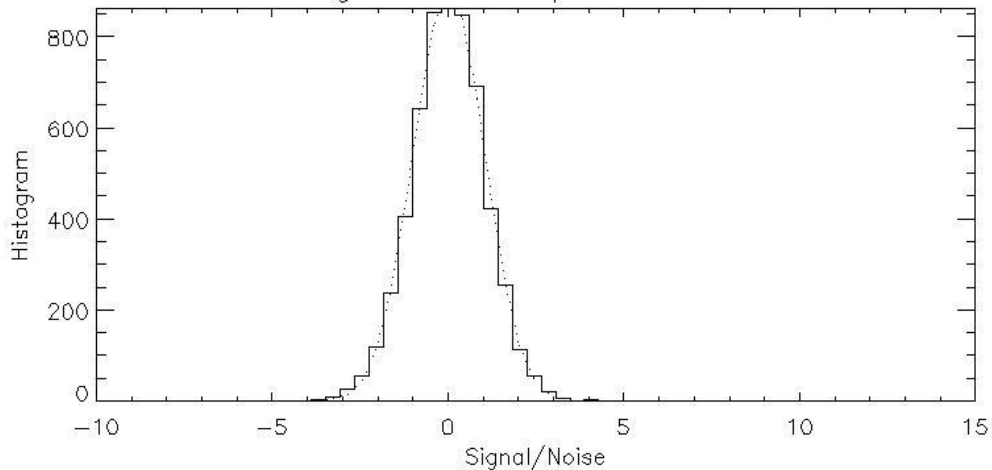
Average RFA Azel Map: PSS2322+1944
