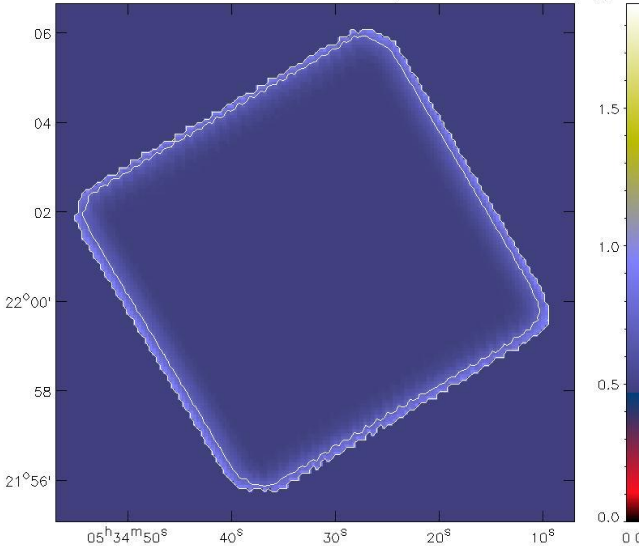
Noise 1mm RF Radec Map: Crab
