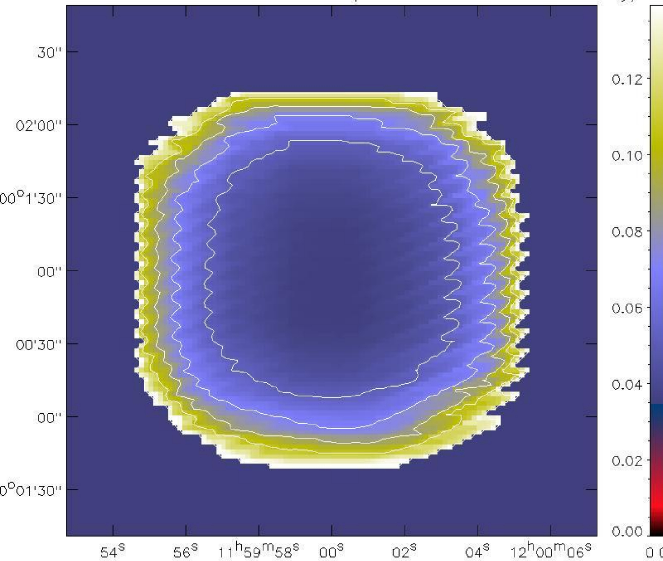
Noise 1mm RF Azel Map: PSS2322+1944
