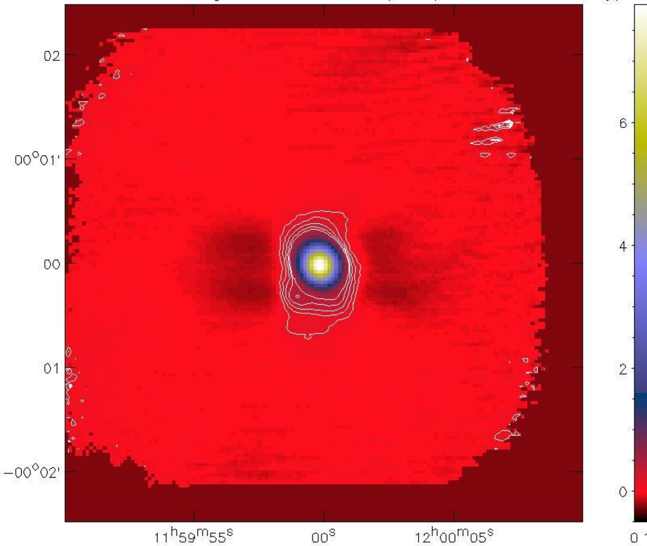
Average 2mm RF Azel Map: Neptune
