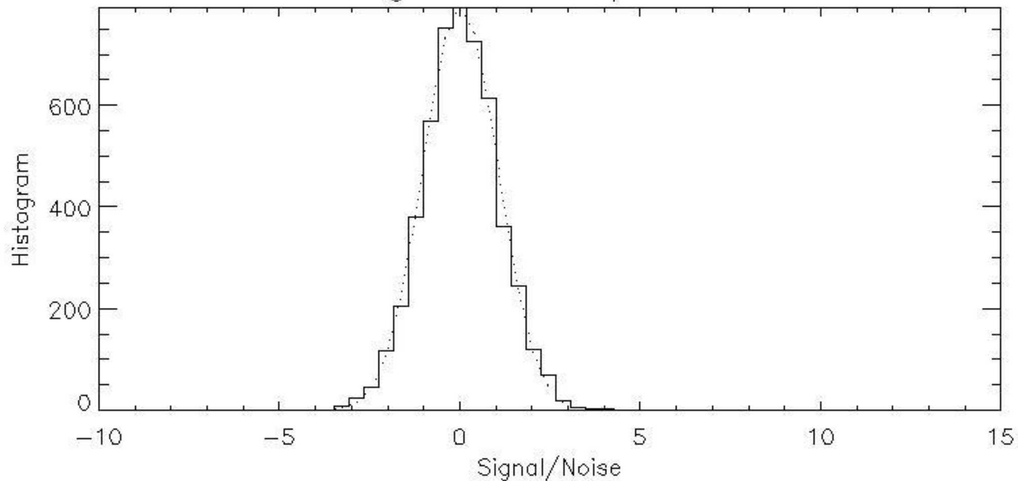
Average RFA Azel Map: IRC10420
