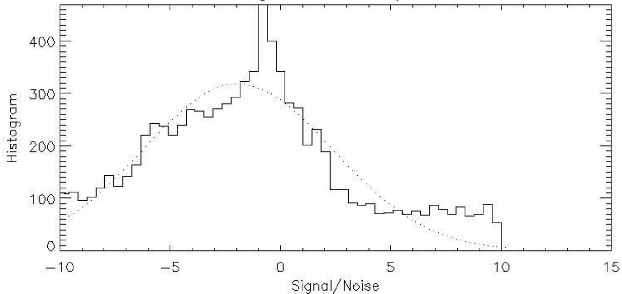
Average RFB Azel Map: Crab
