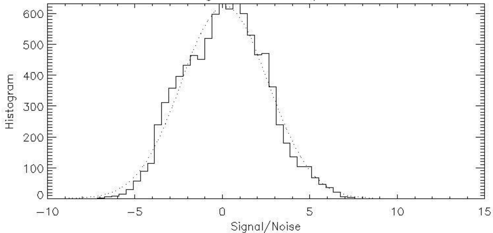
Average RFA Azel Map: Crab
