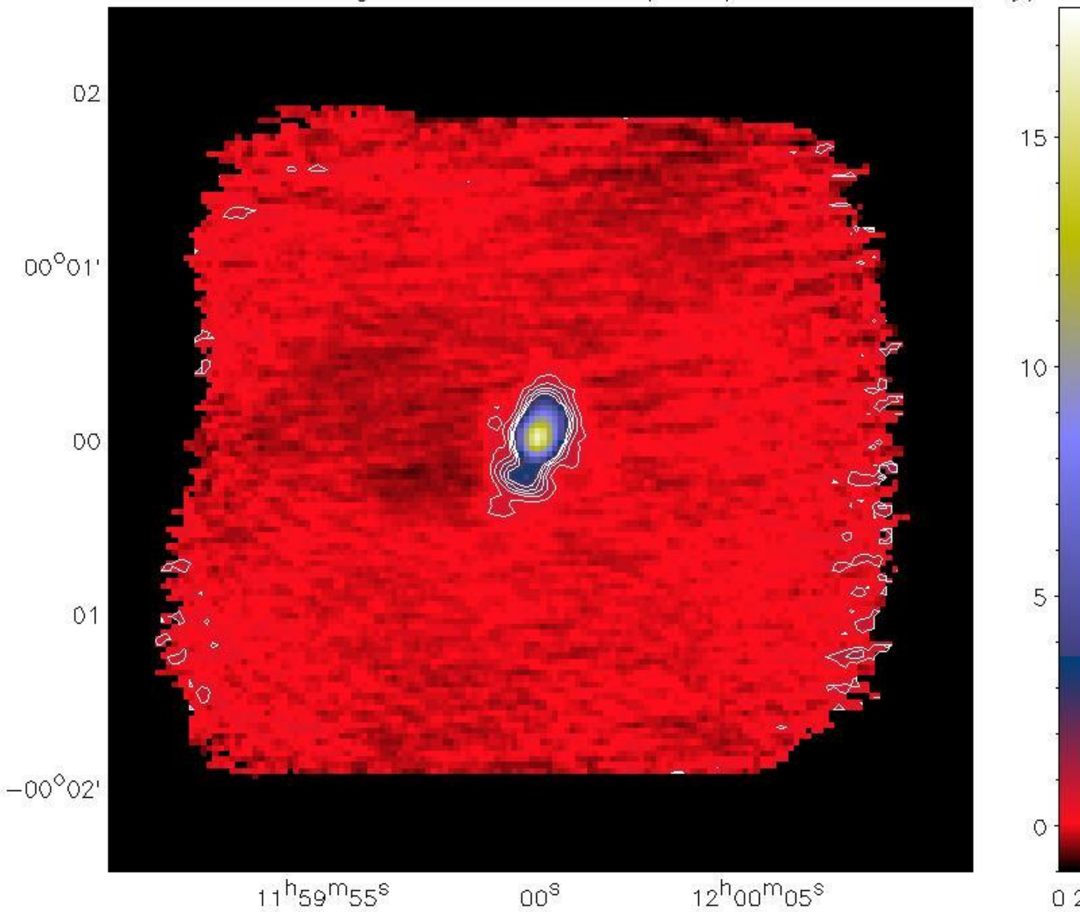
Average 1mm RF Azel Map: Neptune
