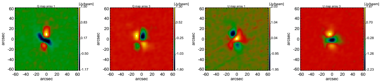
Figure 6: From left to right. Uranus Q array 1, array 3, U array 1, array 3 scan 233. Elevation=55
