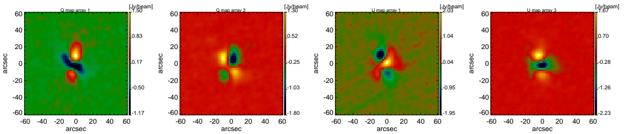
Figure 1: From left to right. Uranus Q array 1, array 3, U array 1, array 3 scan 209. Elevation=58
