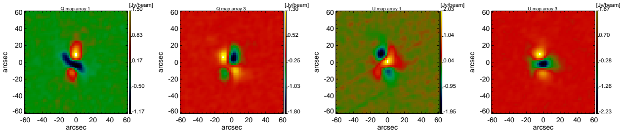
Figure 4: From left to right. Uranus Q array 1, array 3, U array 1, array 3 scan 226. Elevation=54
