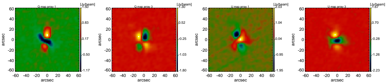
Figure 3: From left to right. Uranus Q array 1, array 3, U array 1, array 3 scan 205. Elevation=31
