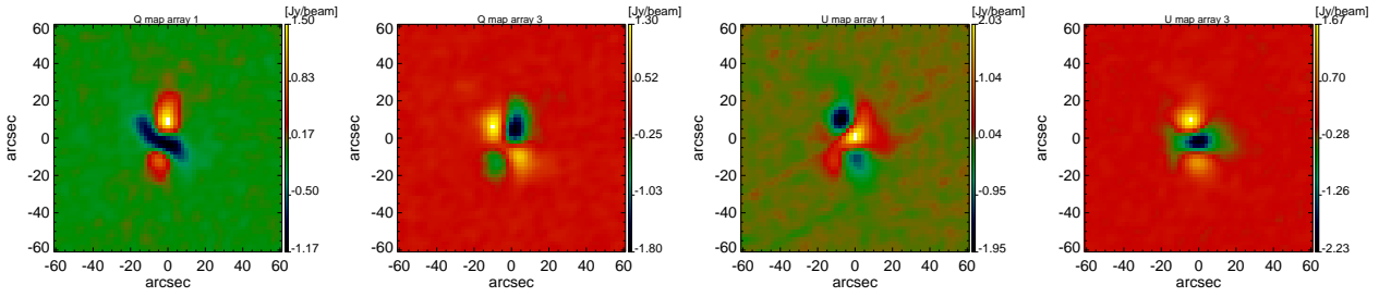
Figure 5: From left to right. Uranus Q array 1, array 3, U array 1, array 3 scan 232. Elevation=57
