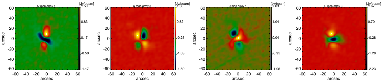
Figure 2: From left to right. Uranus Q array 1, array 3, U array 1, array 3 scan 248. Elevation=54
