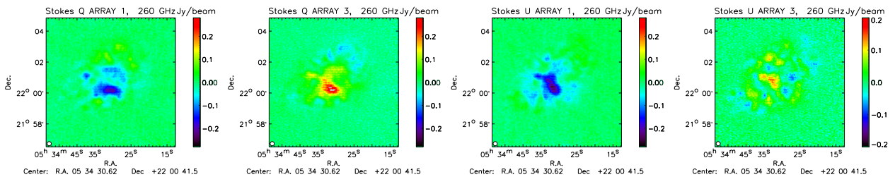
Figure 7: From left to right. CRAB nebula Q array 1, array 3, U array 1, array 3.
