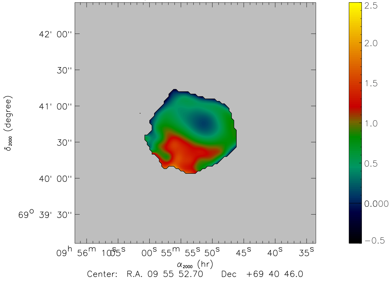
M82 spectral index distribution
