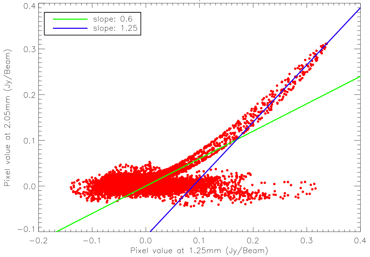
Correlation of the M82 map at 1.25mm and 2.05mm
