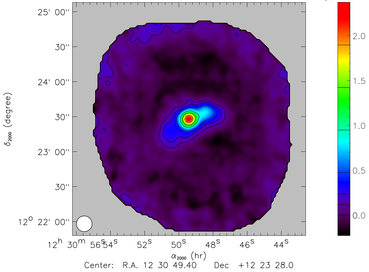
M87 at 1.25 mm
