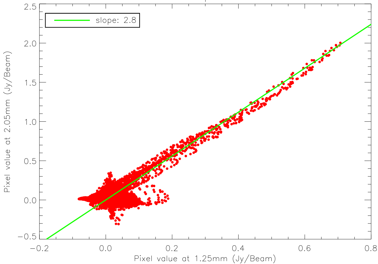
Correlation of the M87 map at 1.25mm and 2.05mm
