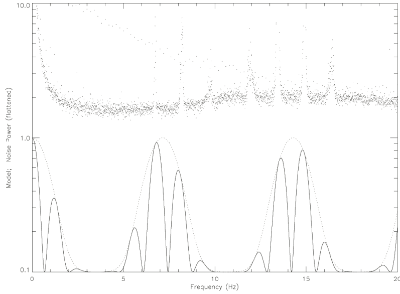
Fig. 4. The dots show the flattened power spectrum with several clear sets of bands. The same data are displayed in all three panels, but on different frequency ranges. Some bands are strong enough that they extend beyond the top of the plot. The “model” spectrum indicated by the solid line is constructed \cos(\pi f / 1.352 \text{ Hz})^2 * [\text{III}(7.142 \text{ Hz}) \otimes e^{-0.5f^2 / (1.59 \text{ Hz})^2}] + 0.1 . The dotted line shows the envelope of the \text{III}(7.142 \text{ Hz}) \otimes e^{-0.5t^2 / (1.59 \text{ Hz})^2} modulation.
