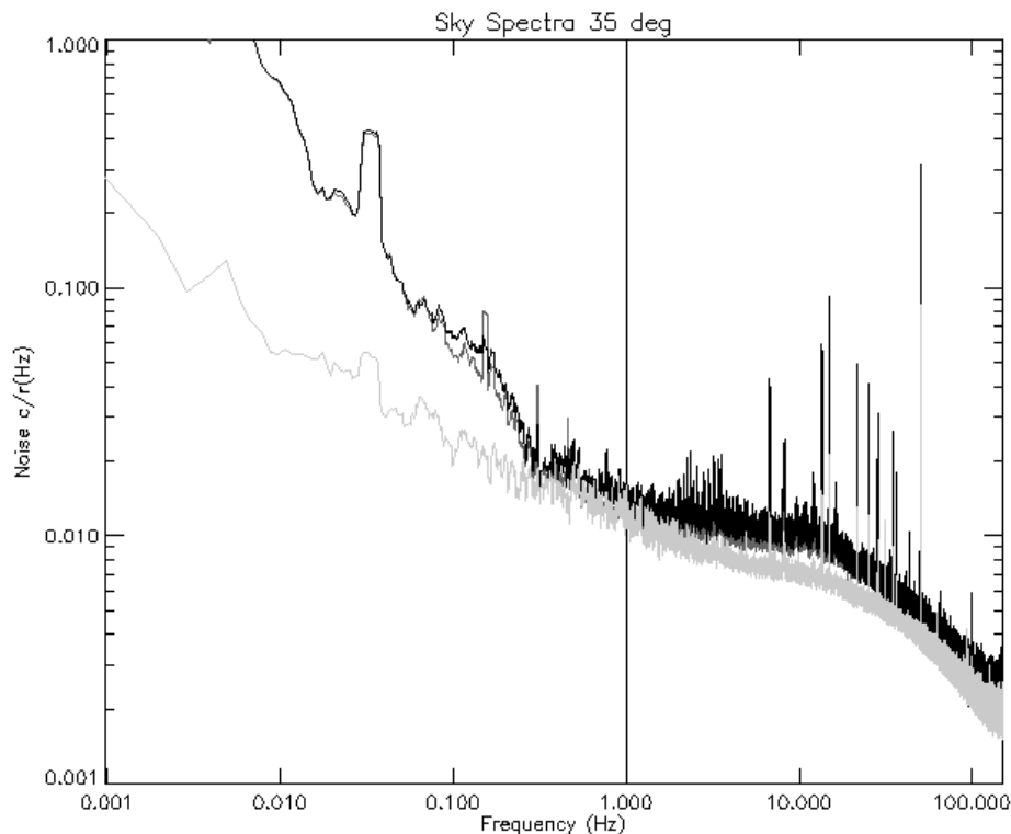
Fig. 3. Raw spectra of detector current noise density of GISMO while installed at the telescope and looking at the sky (dark and medium dark grey: average spectra of working pixels; light grey: average noise spectrum of superconducting (i.e. non biased) detectors.
