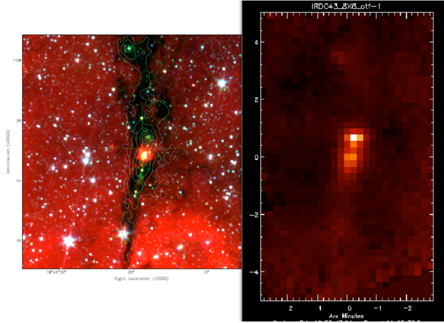
Fig. 9. Left: IRAC Glimpse N3-color IR image of the Infrared Dark Cloud IRDC43 with superimposed Mambo 1.2 mm contours (J. Jackson, priv. comm.). Right: GISMO's view of IRDC 43.
