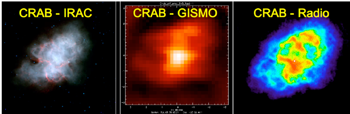
Fig. 8. The CRAB Nebula -- the result of a Supernova explosion -- (left) in the infrared seen by the IRAC, center at 2mm as observed with GISMO, and at centimeter wavelengths as observed by the VLA.
