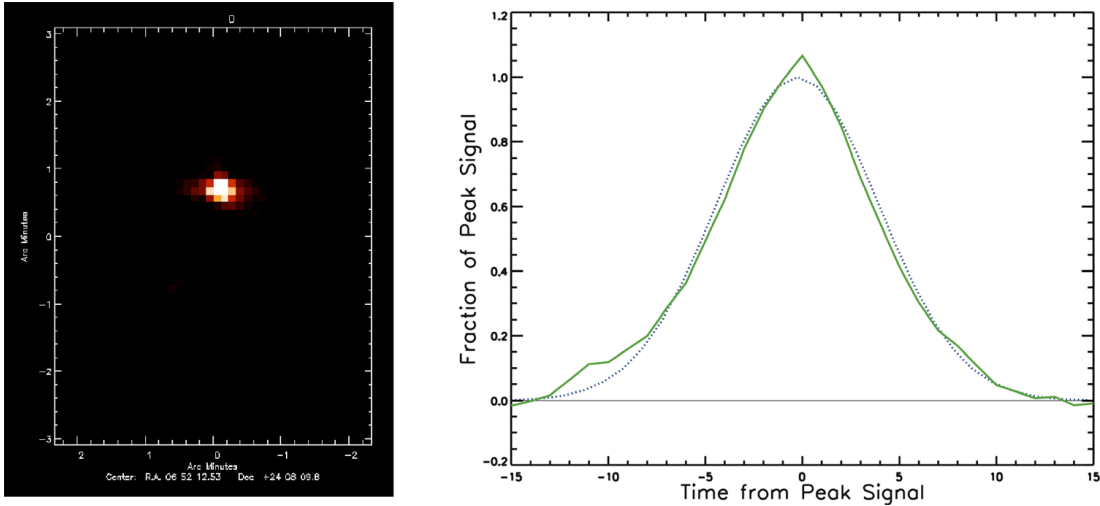
Fig. 5. Left : observation of the planet Mars. The fitted beam size is 21'' \times 15'' . This measurement represents the most extreme beam asymmetry we observed during measurements of point sources. Right : measured azimuthal beam shape derived from observations of Uranus (solid line), superimposed on a Gaussian distribution (dotted line).
