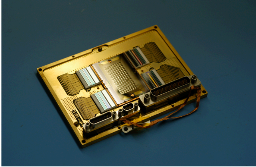
Fig. 1. The GISMO 8x16 planar array in the detector package. SQUID multiplexers, shunts and Nyquist inductors are integrated in the package.
