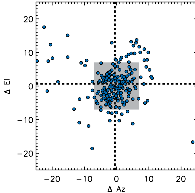
Figure 5: Pointing corrections applied during the GISMO pool. The gray shaded area represents the GISMO pixel size. The black dashed lines correspond to the median values found for \Delta Az and \Delta El .
