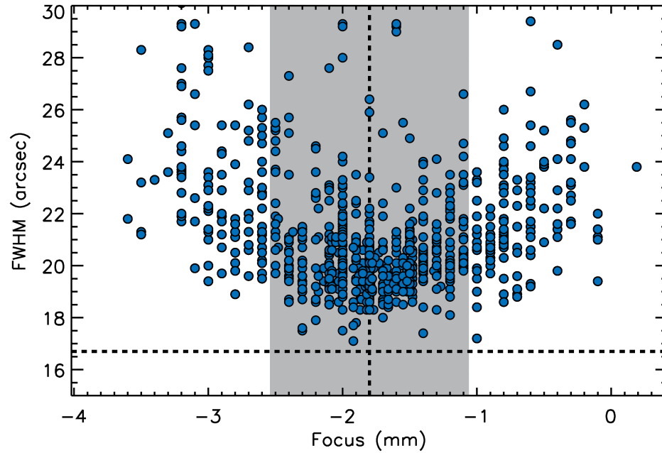
Figure 7: Focus corrections used during the GISMO pool. The vertical black dashed line and the gray shaded area correspond to the median value and to the rms, respectively. The horizontal black dashed line corresponds to the half-power beamwidth of the telescope ( 16.7'' ).
