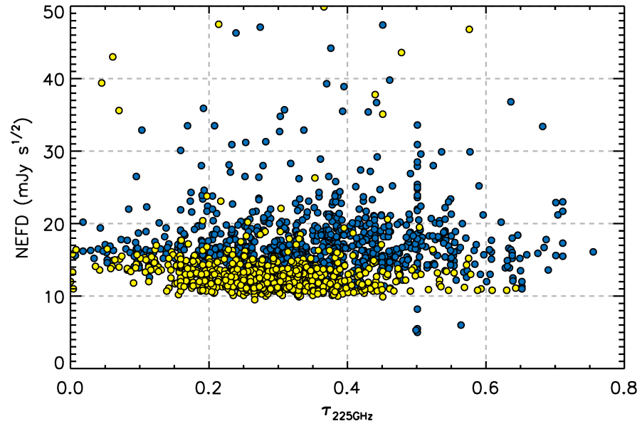
Figure 4: Trend of the NEFD with the opacity for the cases of a scan speed lower (blue) and greater (yellow) than 60''/s
