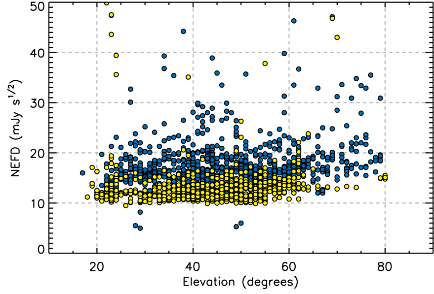
Figure 3: Trend of the NEFD with the elevation for the cases of a scan speed lower (blue) and greater (yellow) than 60''/s
