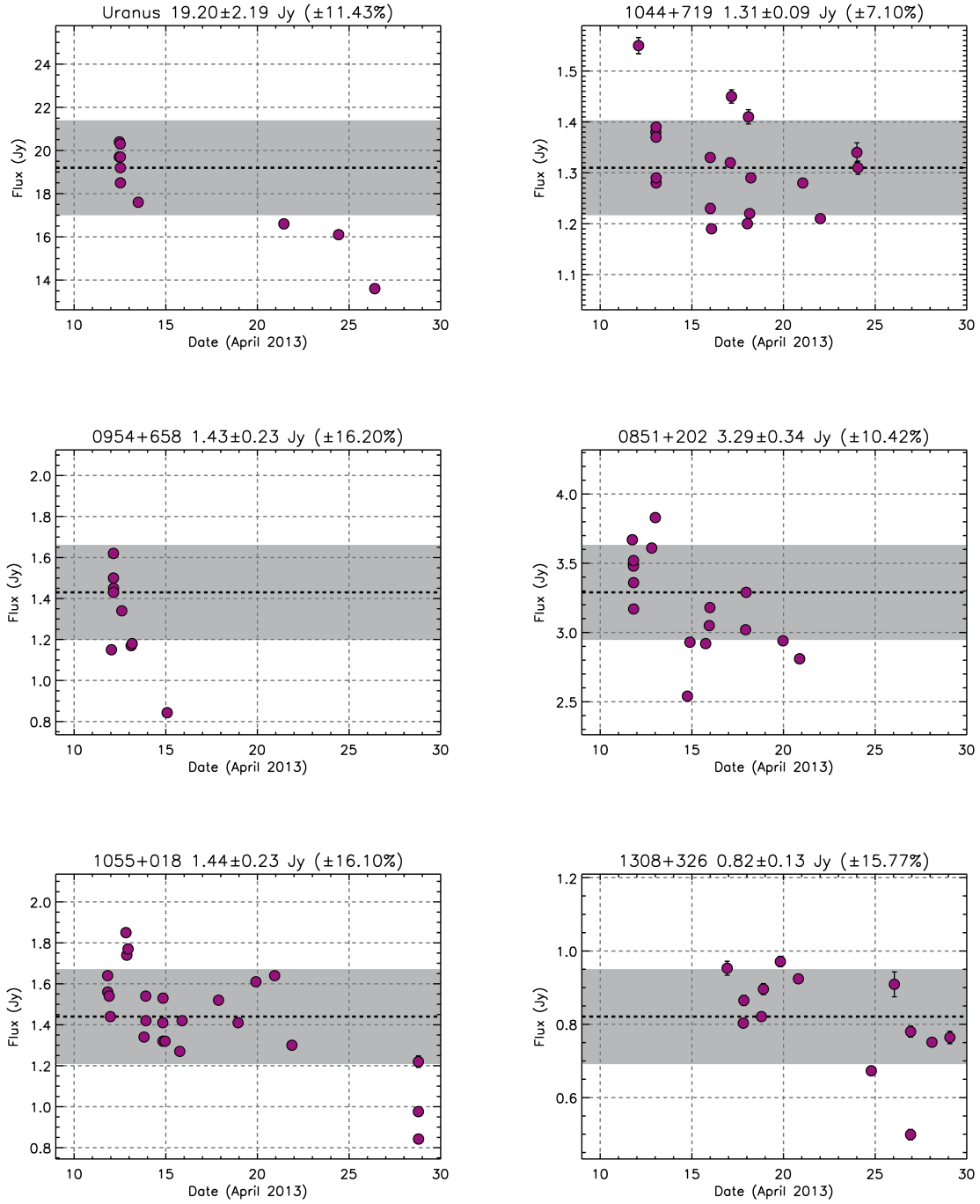
Figure 9: Flux of the pointing sources vs date. The black dashed and the gray shaded area correspond to the median value and to the rms, respectively.
