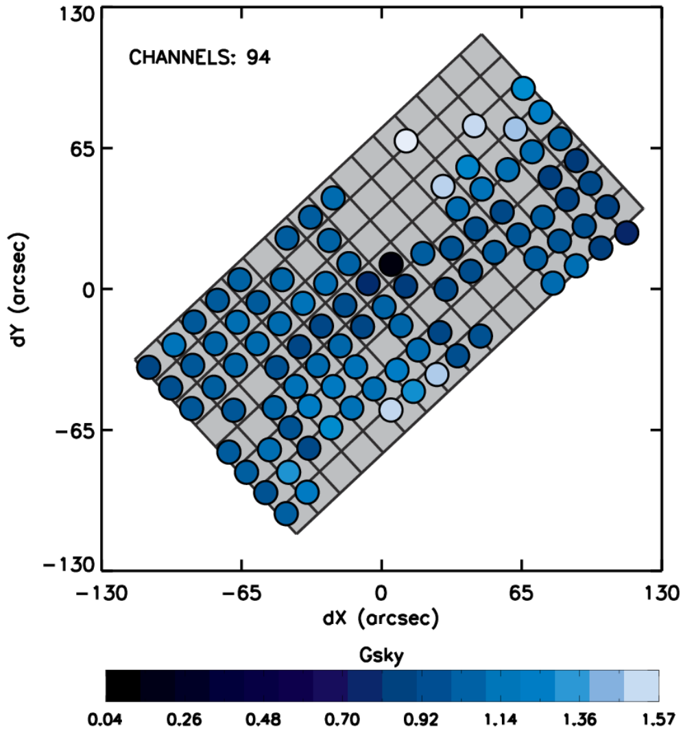
Figure 10: Pixel position in the field of view (filled circles) and sky gain (color code) obtained for one of the beam maps taken during the 3rd GISMO pool. The GISMO array (gray shaded grid) has been included for reference.
