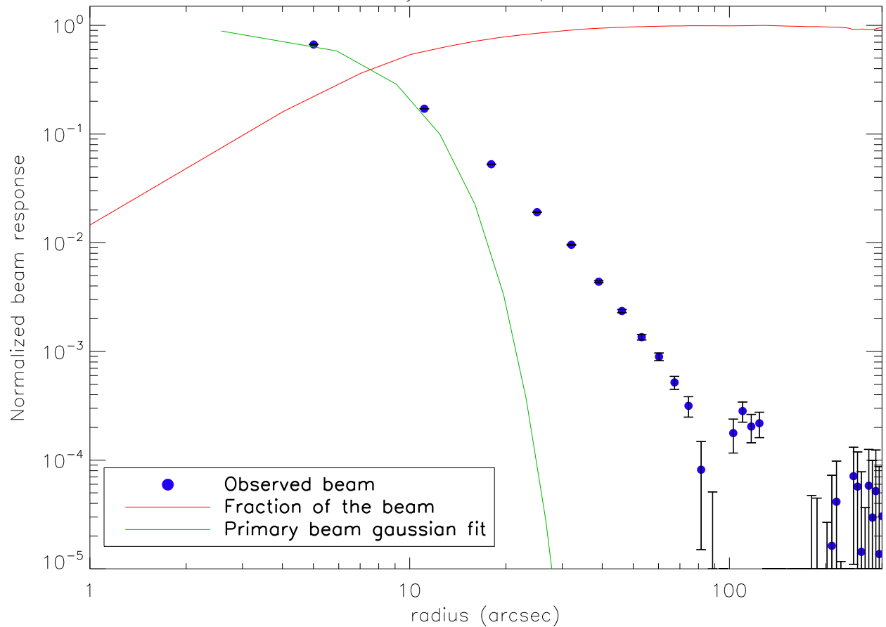
Array 3 beam profile
