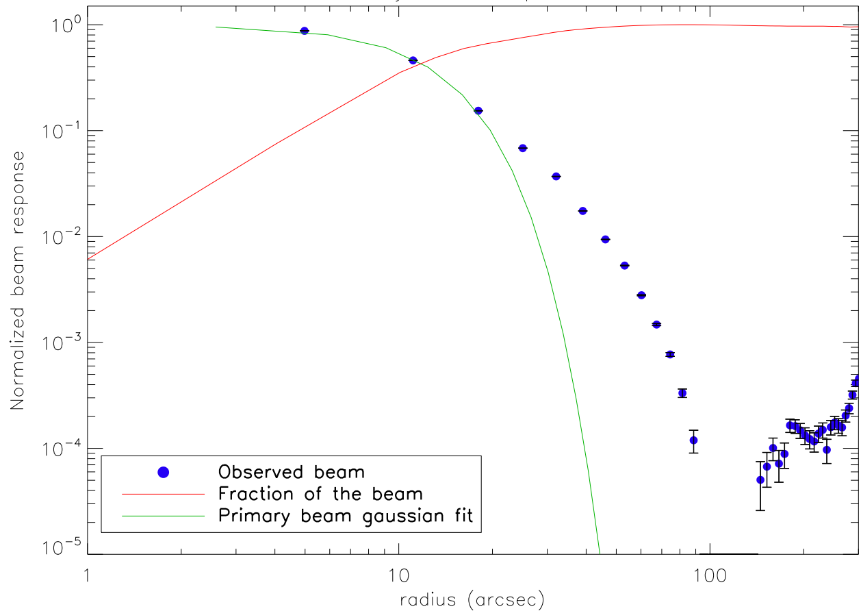
Array 2 beam profile
