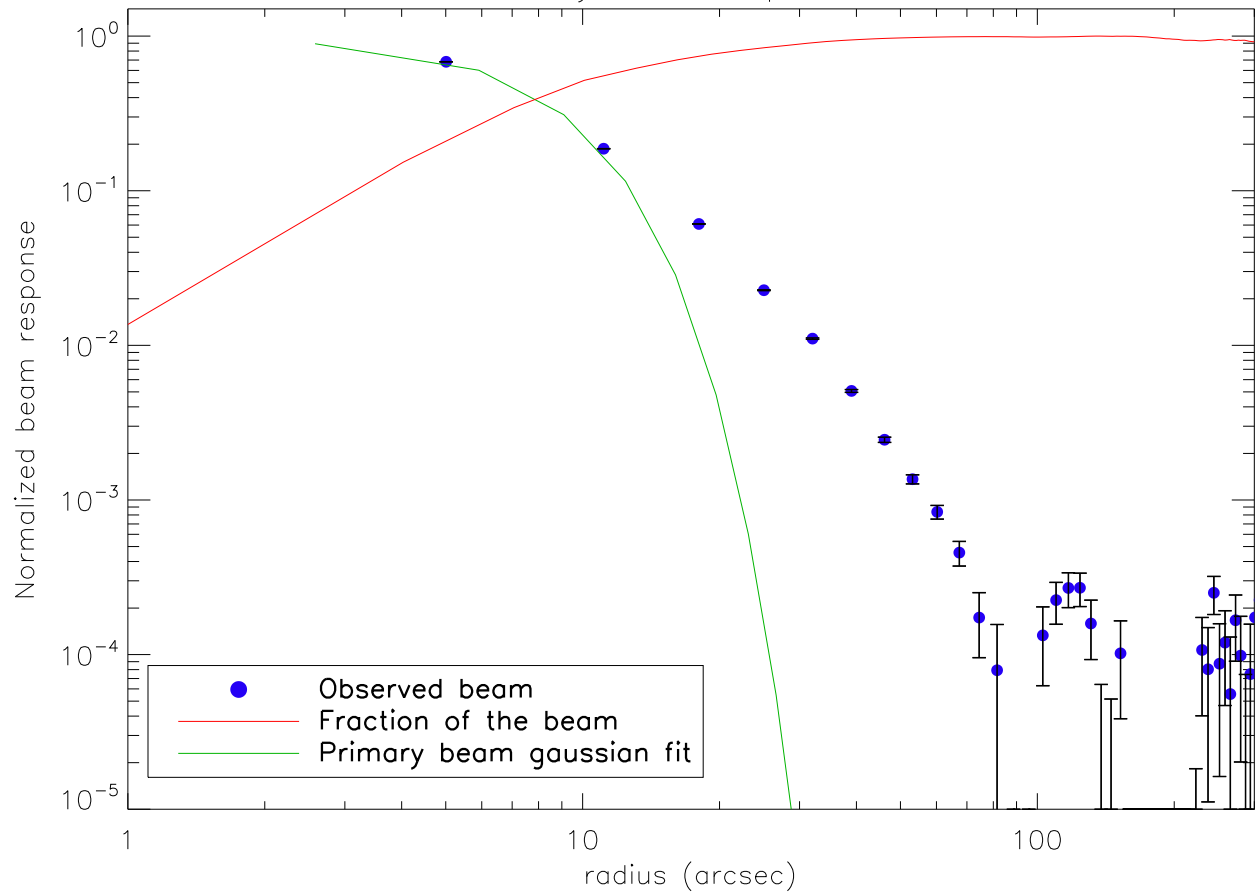
Array 1 beam profile
