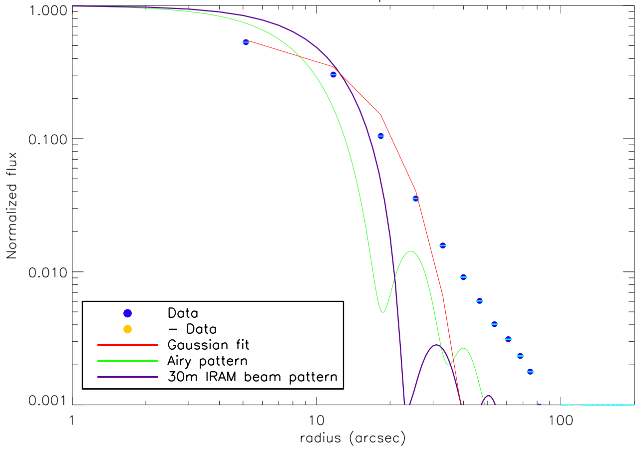
Saturn – normalized profile at 2 mm
