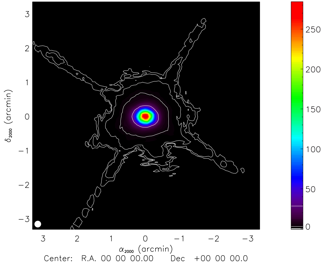
Saturn at 2.05 mm
