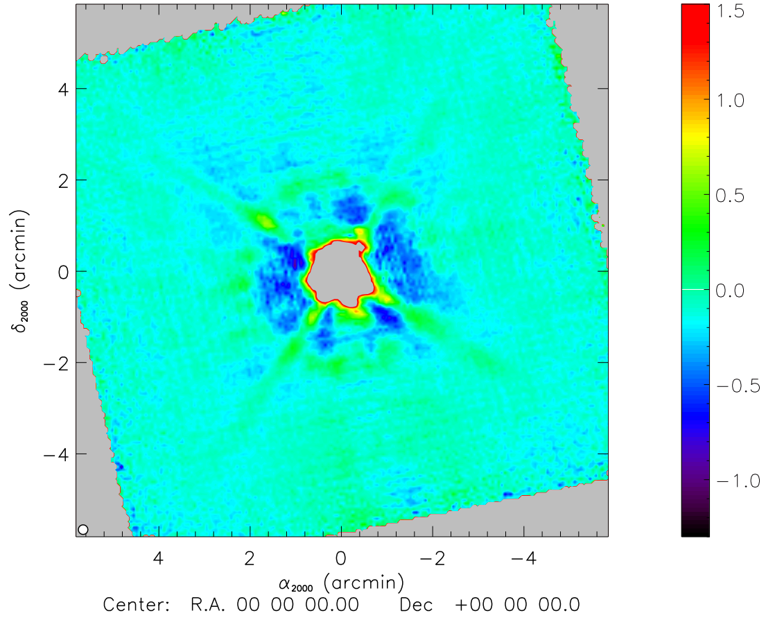
Saturn at 1.25 mm
