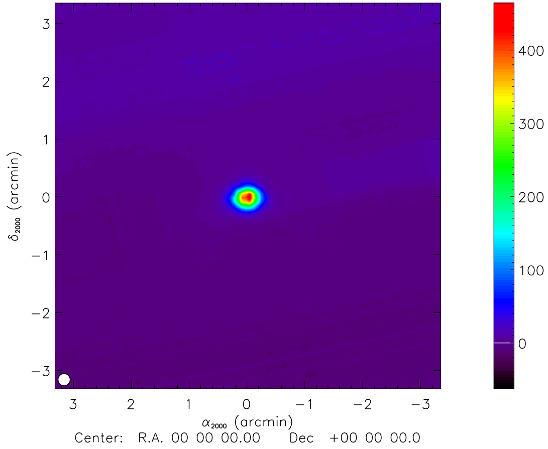
Saturn at 1.25 mm
